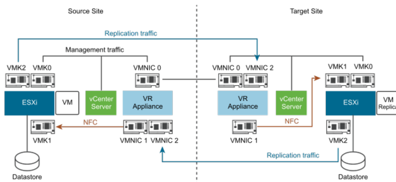
Figure 5: vSphere Replication Traffic Isolation
